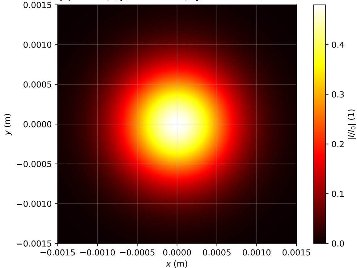
Intensity profile I(x, y, z = 2.707m)/I_0 , Pin=0.3Pcr, artificial time
